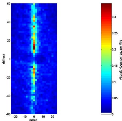
Figure 14B: Relative aircraft density for Logen Sector (Transition sector).
