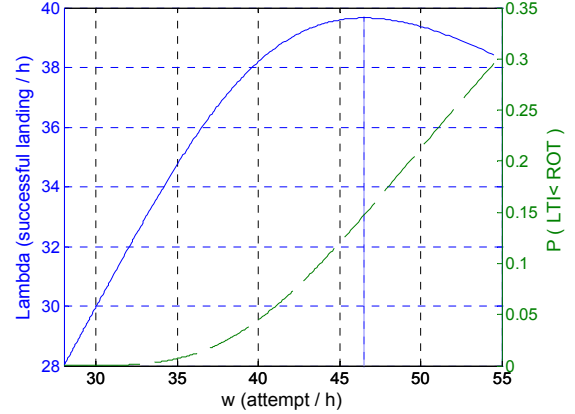
Figure 4. Landing/h (left) and P\{GA\} (right) vs. Attempts/h ( \omega )
